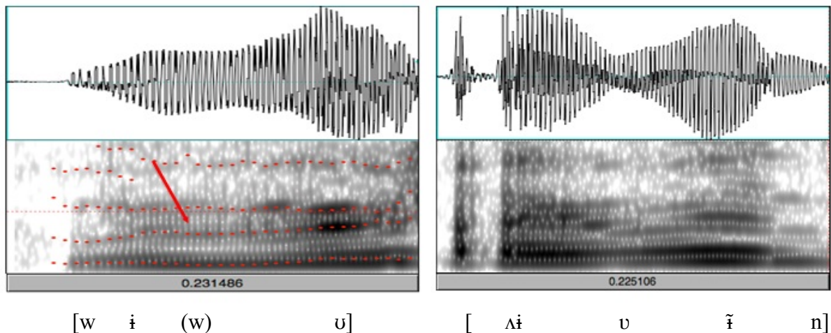
Fig. 1. Waveforms and spectrograms, with formant overlay, of we were (left panel) and I haven't (right panel) from a casual conversation. The arrow in the left panel indicates a slight dip in F2 that may reflect a second /w/.
